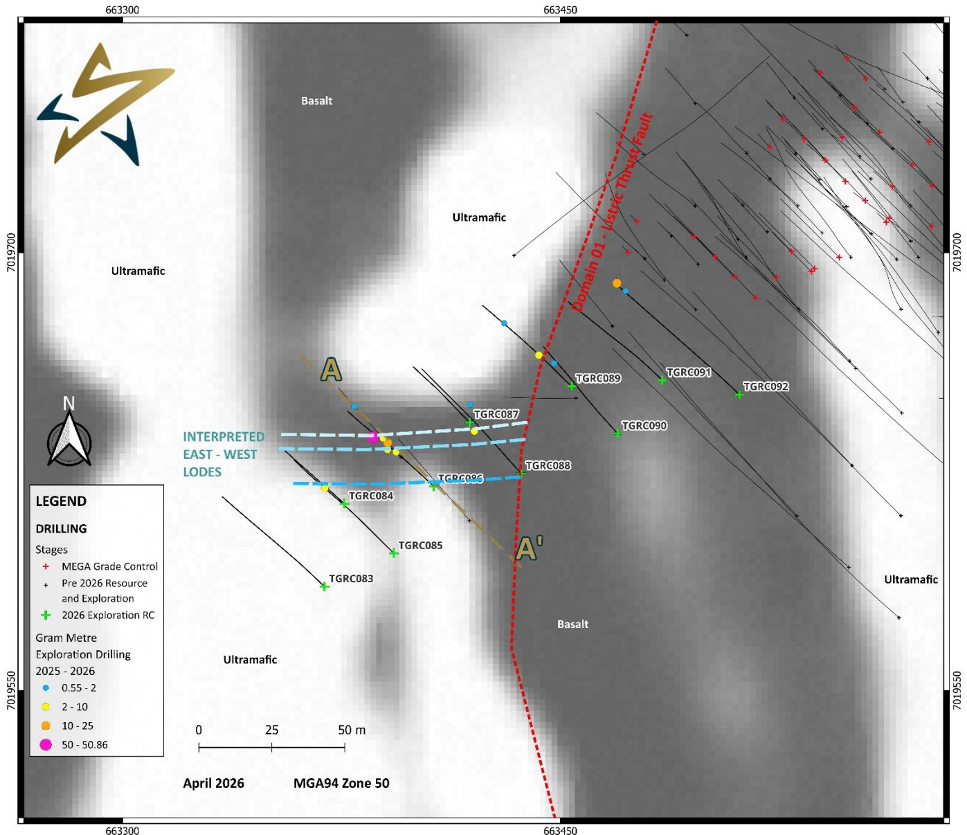
Figure 3: Western Area Mineralisation Interpretation
